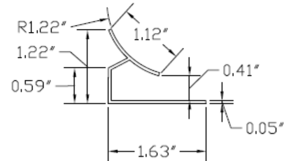
Inside Corner
