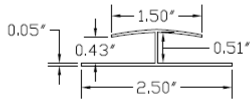
H Divider
