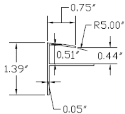
F Profile
