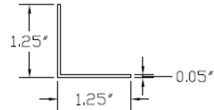
Outside Corner
