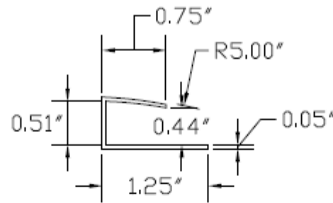
J Trim
