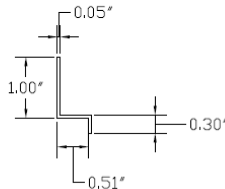
Base Trim
