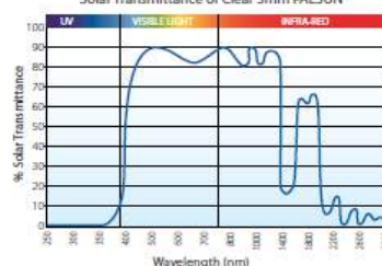
Solar Transmittance of Clear 3mm PALSUN®
